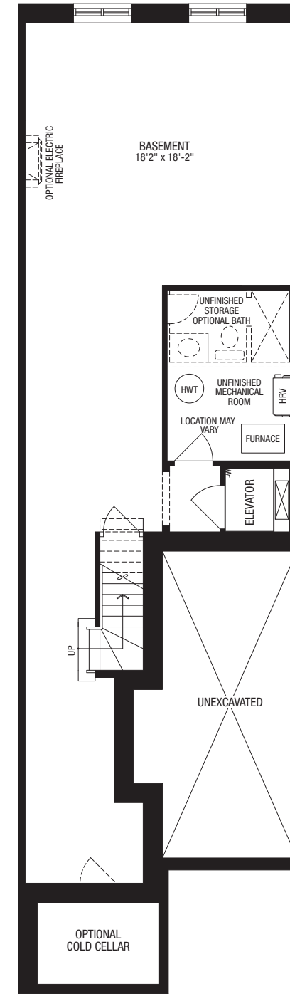
OPTIONAL ELEVATOR BASEMENT PLAN ELEV. 'A' & 'B' (ELEV. 'C' SIMILAR)
