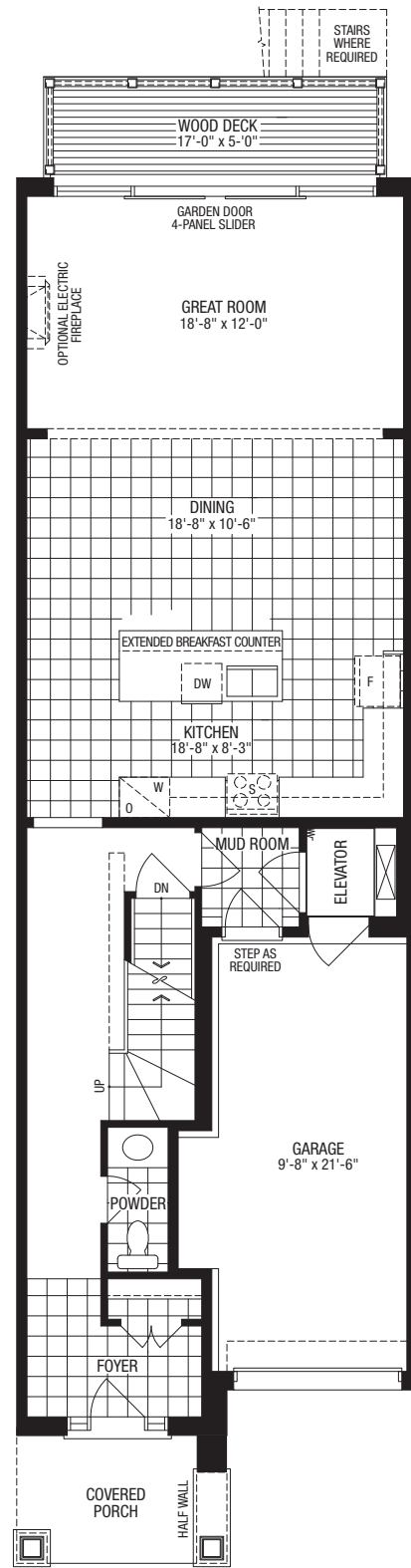
OPTIONAL ELEVATOR GROUND FLOOR PLAN ELEV. 'A' & 'B' (ELEV. 'C' SIMILAR)
