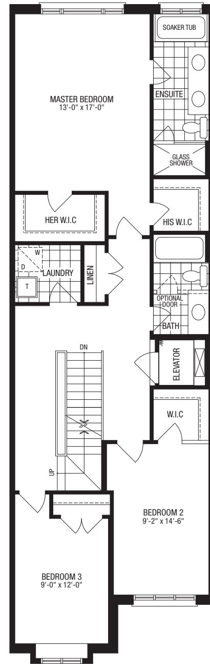
OPTIONAL ELEVATOR SECOND FLOOR PLAN ELEV. 'A' & 'B' (ELEV. 'C' SIMILAR)
