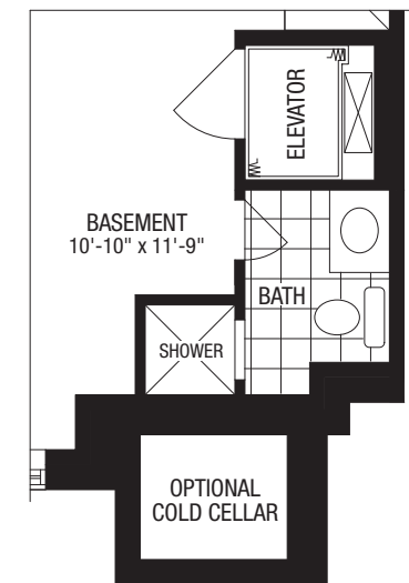
PARTIAL OPTIONAL ELEVATOR BASEMENT PLAN WITH BATHROOM ELEV. 'A' ('B' SIMILAR)
