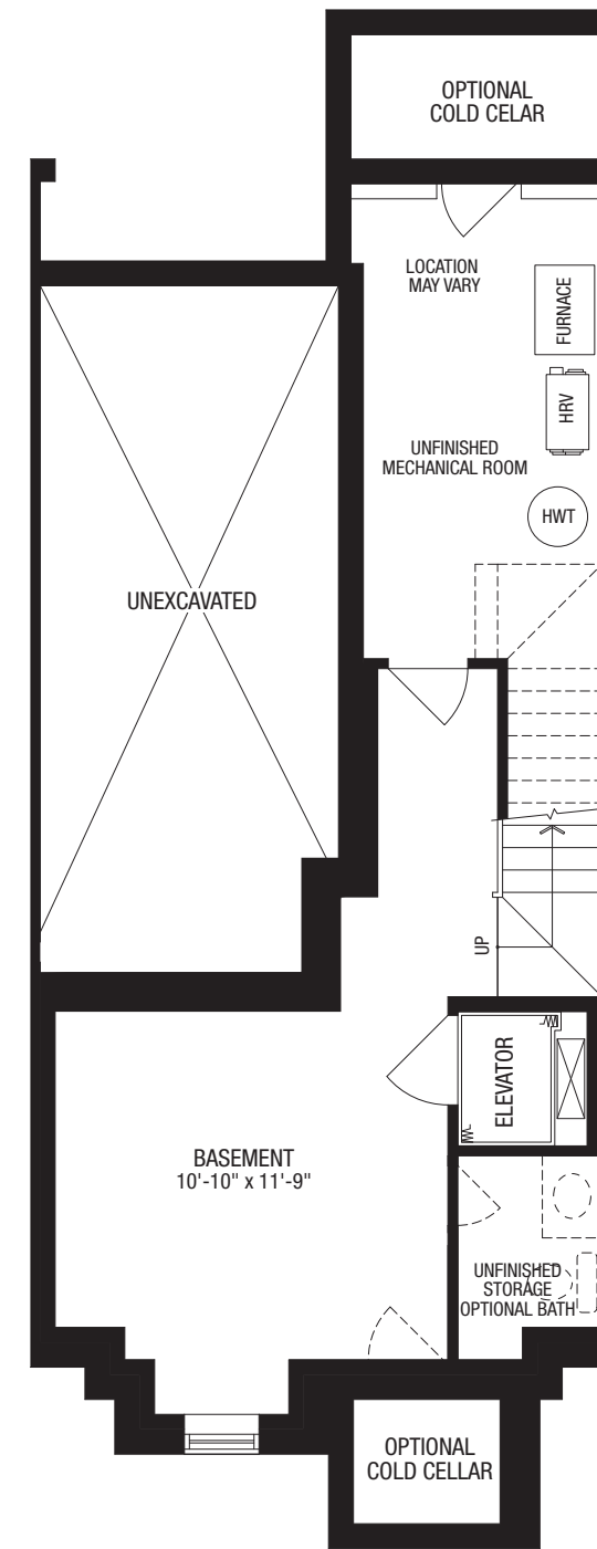
OPTIONAL ELEVATOR BASEMENT PLAN ELEV. 'A' ('B' SIMILAR)
