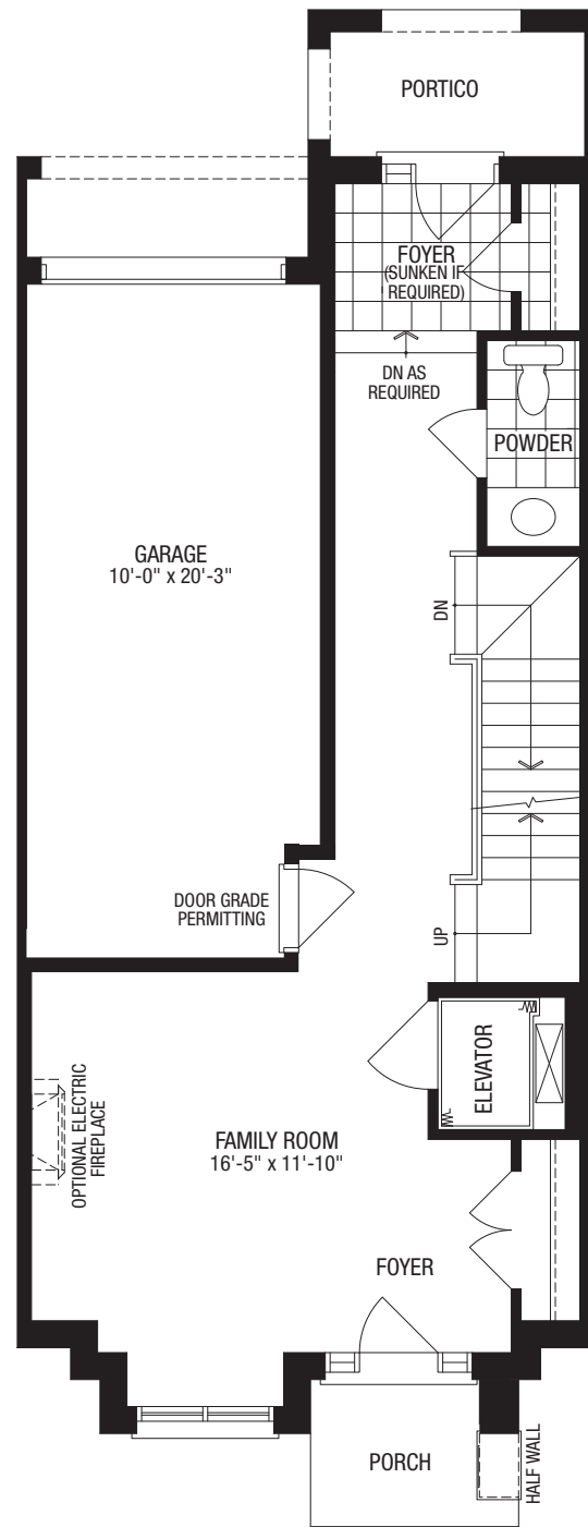
OPTIONAL ELEVATOR GROUND FLOOR PLAN ELEV. 'A' ('B' SIMILAR)
