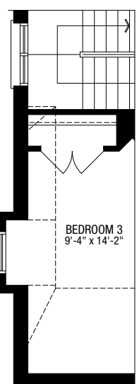
PARTIAL THIRD FLOOR PLAN ELEV. 'B' CORNER UNIT - LOT 1
