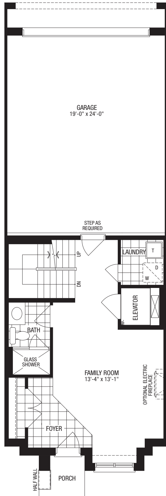
OPTIONAL ELEVATOR GROUND FLOOR PLAN ELEV. 'A', ('B' SIMILAR)
