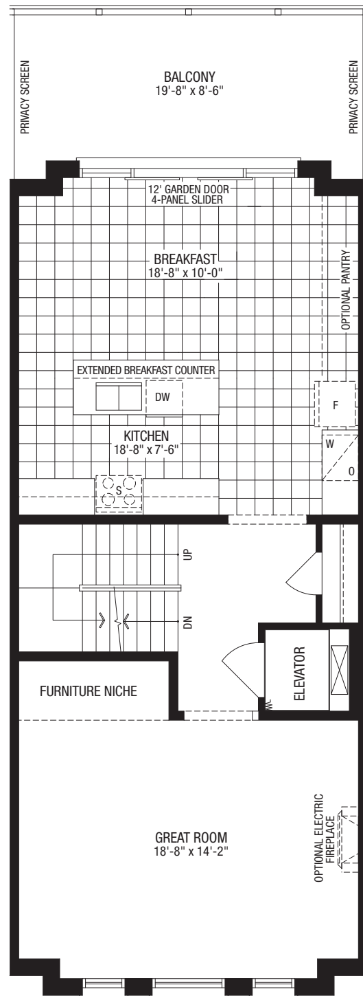
OPTIONAL ELEVATOR SECOND FLOOR PLAN ELEV. 'A', ('B' SIMILAR)
