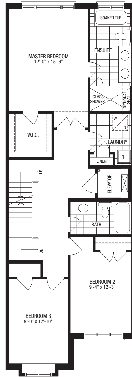
OPTIONAL ELEVATOR SECOND FLOOR PLAN ELEV. 'A' & 'B' ('C' SIMILAR)
