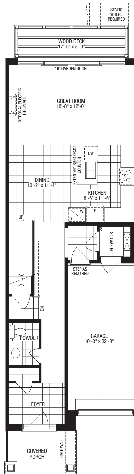
OPTIONAL ELEVATOR GROUND FLOOR PLAN ELEV. 'A' & 'B' ('C' SIMILAR)
